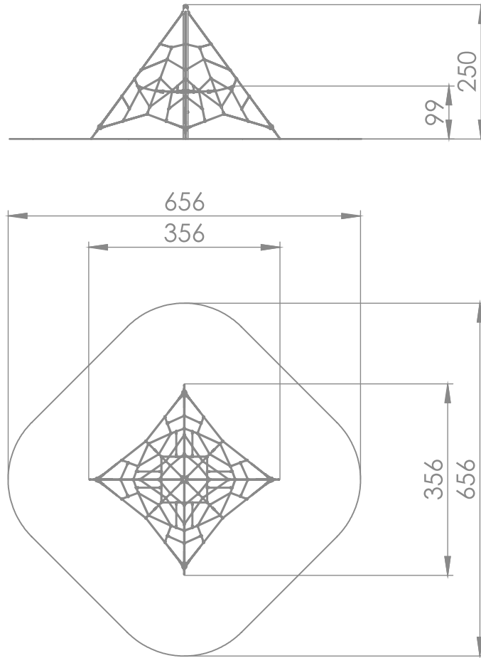
SCALE 1:100
